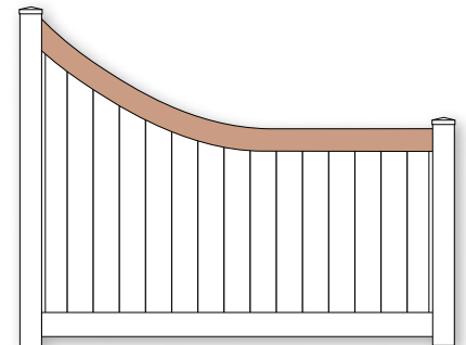
SWEEP "I" RAIL
