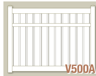
V500A SEMI-PRIVACY WITH ALTERNATING 6" AND 1-1/2" BOARDS
