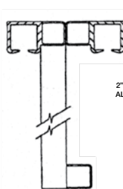
Dual Track Single Gate 31'-0" to 40'-0"
